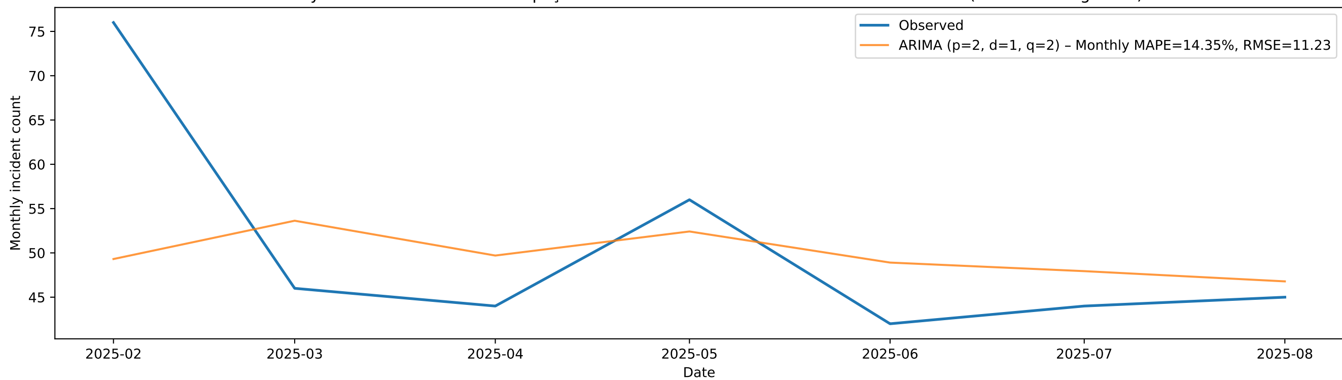
Monthly Traffic Incidents in Mürselpaşa Boulevard: Best Time-series Model vs Observed (Feb 2025-Aug 2025)
